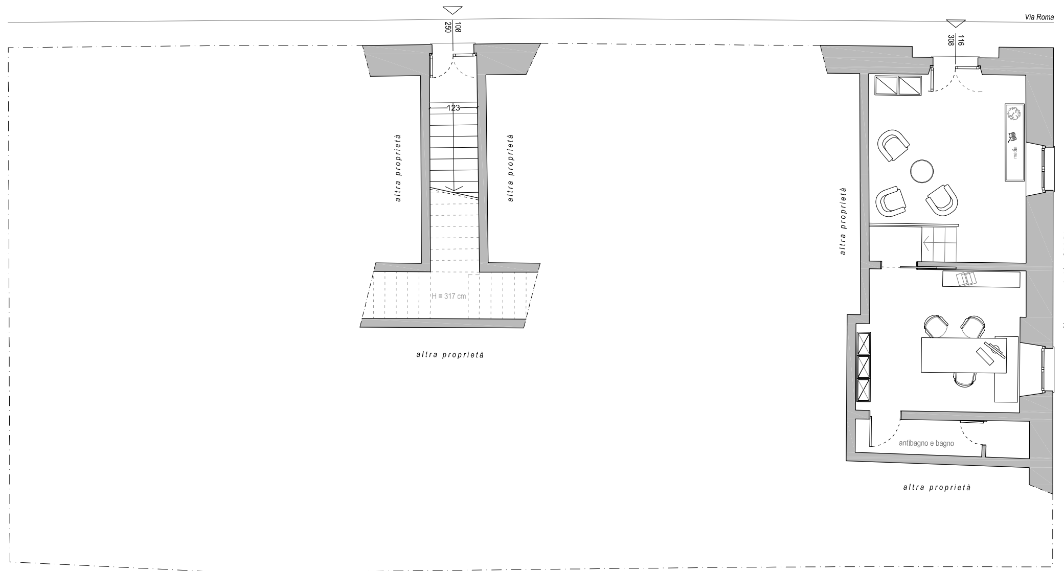
PIANO TERRA scala 1:100
